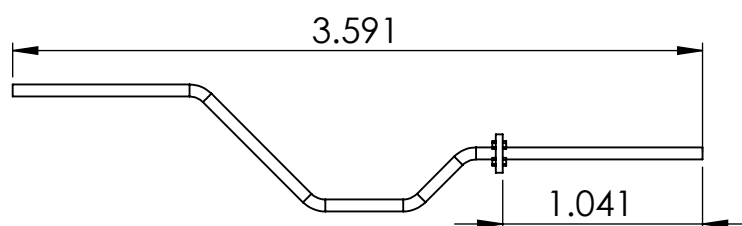
Top feed injector pipe - full size.
